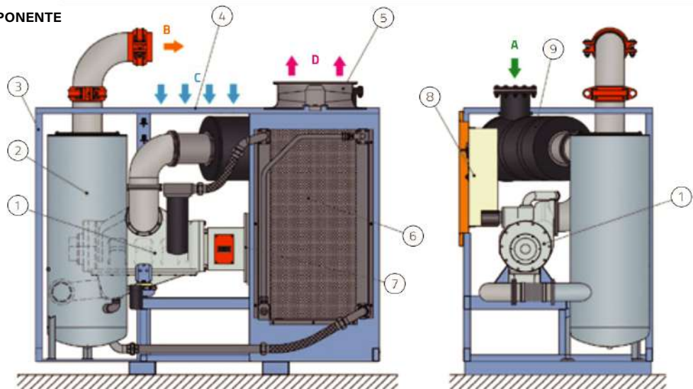
UV30 - UV50 layout
